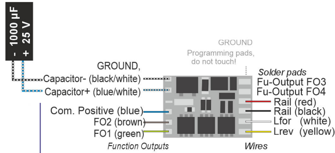
Connection diagram MX671, MX671R Connection Side
