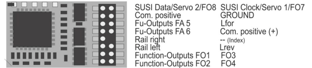
Connection diagram MX685P16 Pad assignment
