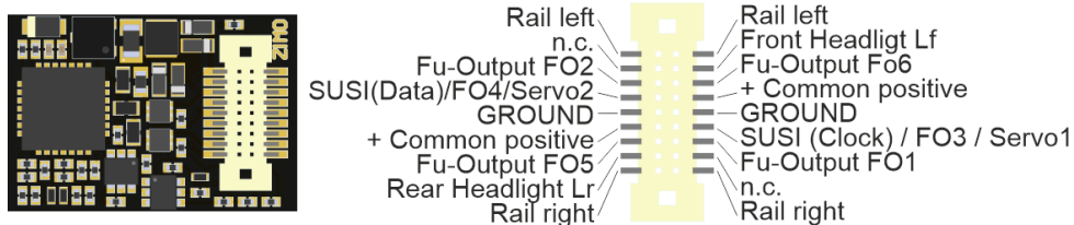
Connection diagram MX689N18 Plug Side View (Next-18)
