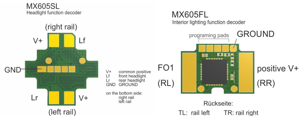
Connection diagram MX605SL and MS605FL - KATO models
