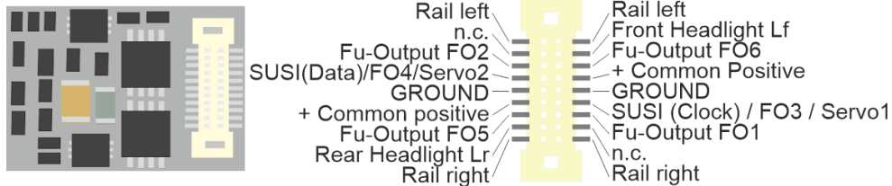
Connection diagram MX688N18 Plug Side View (Next-18) (Replaced by MX689N18)
