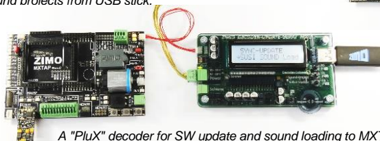
A "PluX" decoder for SW update and sound loading to MXTAPV; connection to MXULFA via "SUSI" cable, but NO cable "rail" from MXULFA to TAP!
