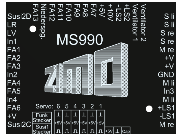
The base of the large-scale decoder MS990 ▶
